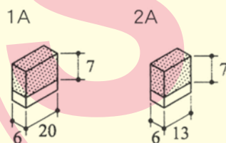
鑽石齒塊尺寸 / The dimensions of diamond tips
