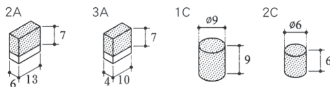
鑽石齒塊尺寸 / The dimensions of diamond tips
